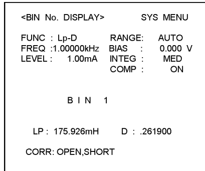
Figure 5. Measurement result using the built-in comparator.
