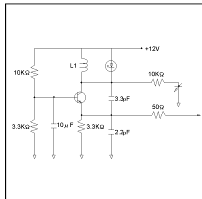
Figure 6. Part of VCO circuit used in a 20 Hz to 30 MHz synthesizer.
